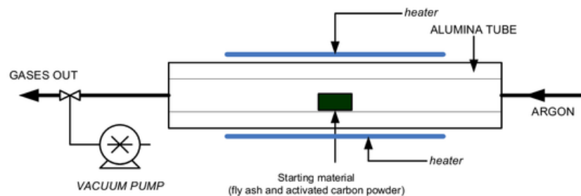
FIGURE 1. Schematic of carbothermal reduction process
