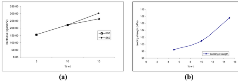
(a) Effect of sintering temperature and % wt of reinforcement on hardness of MMC ALFA (b) Effect of % weight of reinforcement on flexural strength of MMC ALFA at sintering temperature of 550 °C for 2 hours
