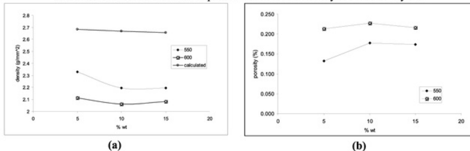
FIGURE 4. (a). Effect of sintering temperature and % wt on density of MMC (b). Porosity of MMC product
