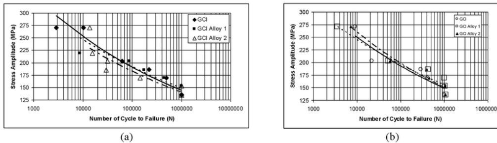
3 Figure 3. Effect of alloy on the fatigue strength of GCI a. at room temperature (35° C), b. at temperature 300° C
