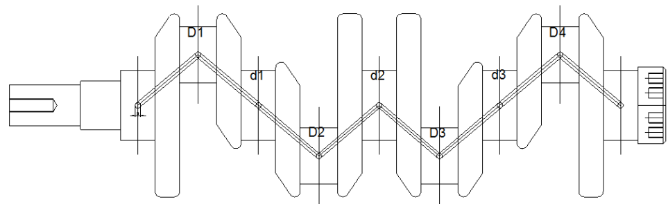
Gambar 3.9. Poros Engkol
