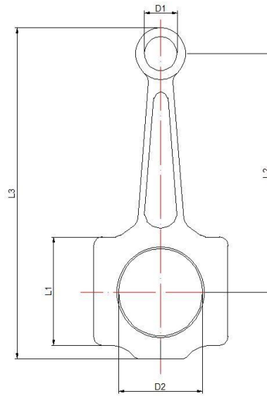
Gambar 3.5. Connecting Rod
