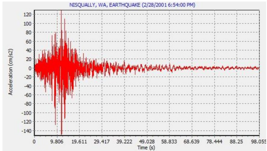
Fig. 3. Time History of Nisqually, Washington (Strong Motion Data Center)
