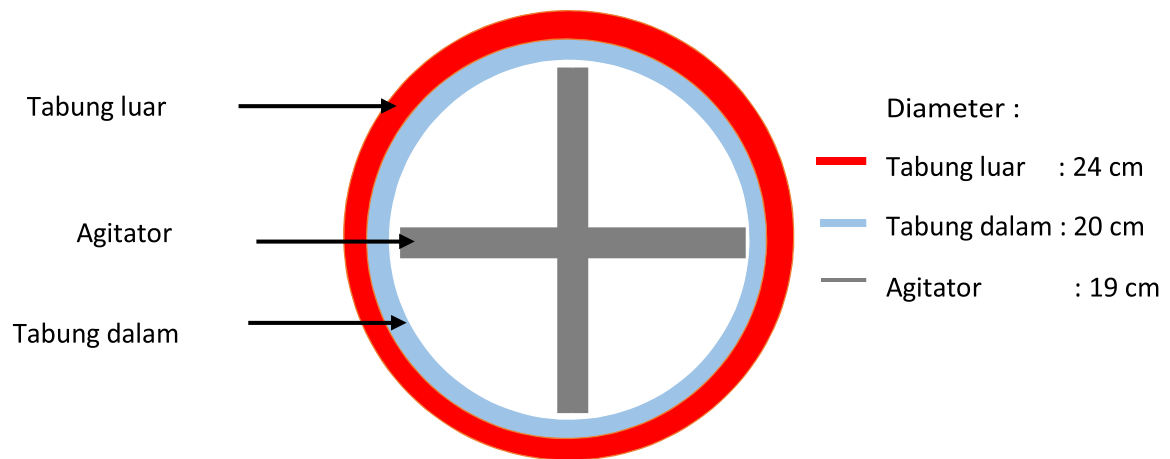
Gambar 10. Diameter Evaporator
