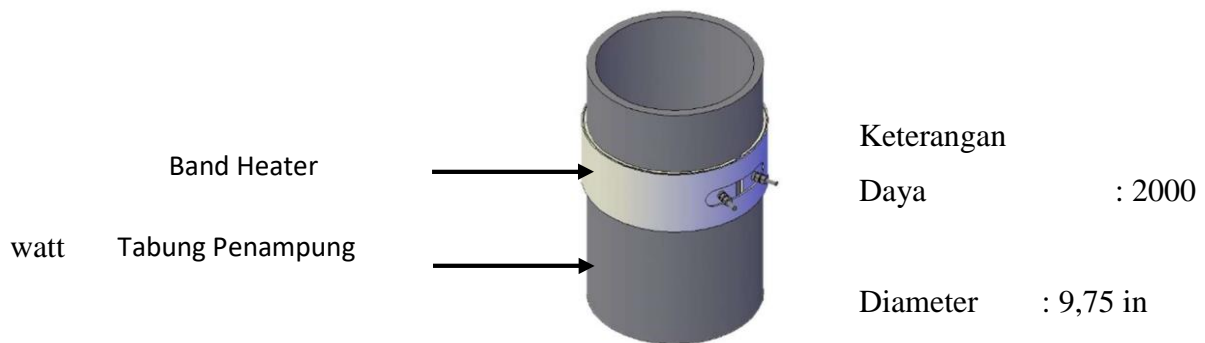
Gambar 11. Band Heater
