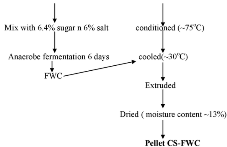
Illustration 2. Diagram process to make pellet of CS-FWC
