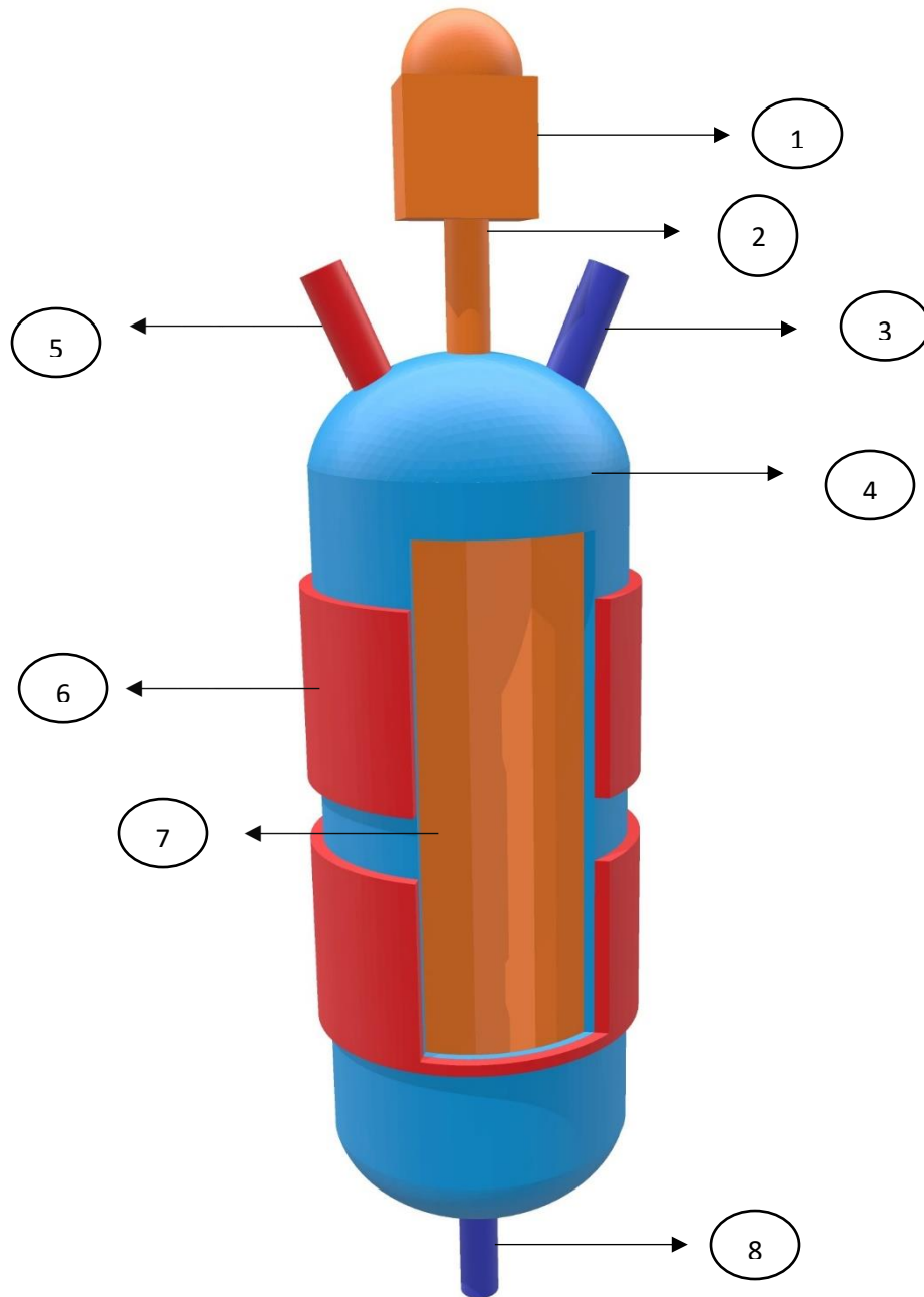
Gambar 9. Agitated Thin-Film Evaporator
