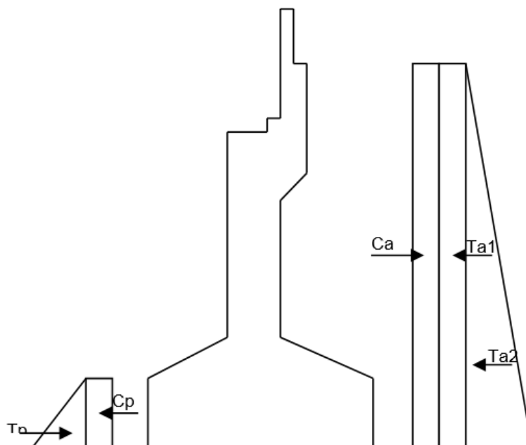
Gambar 2.5 Diagram Tekanan Tanah
