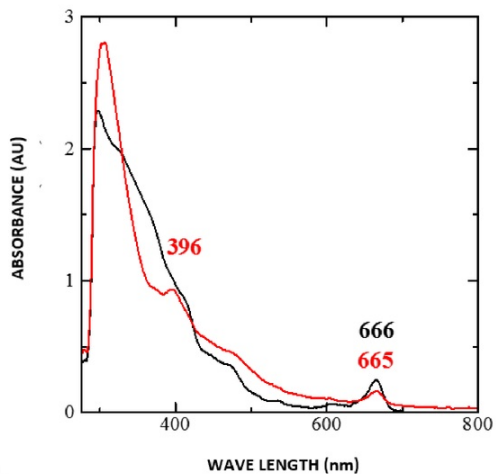
Figure 1. Chlorophyll a and b spectra on leaves and barks of mangrove.
