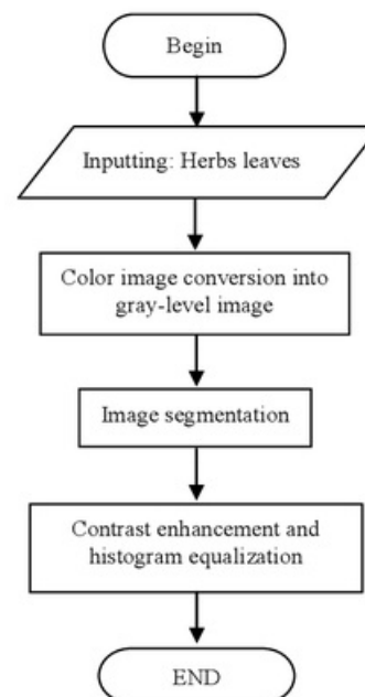
Fig. 1 Preprocessing flowchart
