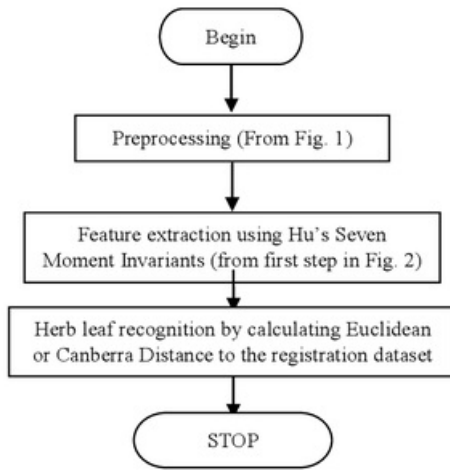
Fig. 3 Herb leaf recognition flowchart
