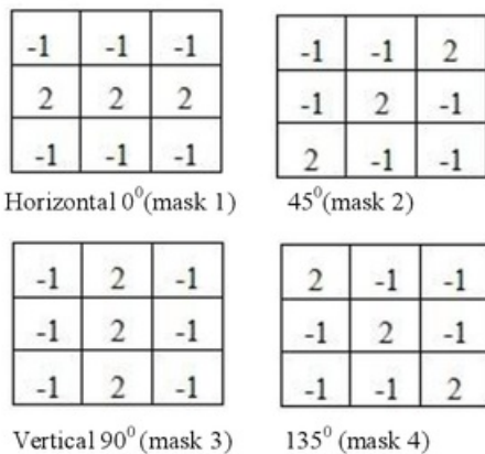
Fig. 2. Masking for 0°, 45°, 90°, 135° directions respectively.
