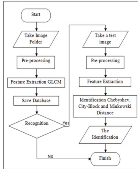
Figure 2. Flowchart of system
