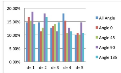
Figure 7. Success Rates Graph of Test Image Recognition Minkowski
