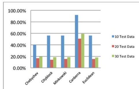
Figure 8. Graph of Success Rate Introduction of 10, 20 and 30 Leaf Types
