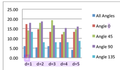
Figure 5. Success Rates Graph of Test Image Recognition using Chebyshev distance
