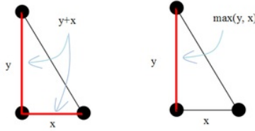
Figure 3. Comparison between City-block and Chebyshev distances
