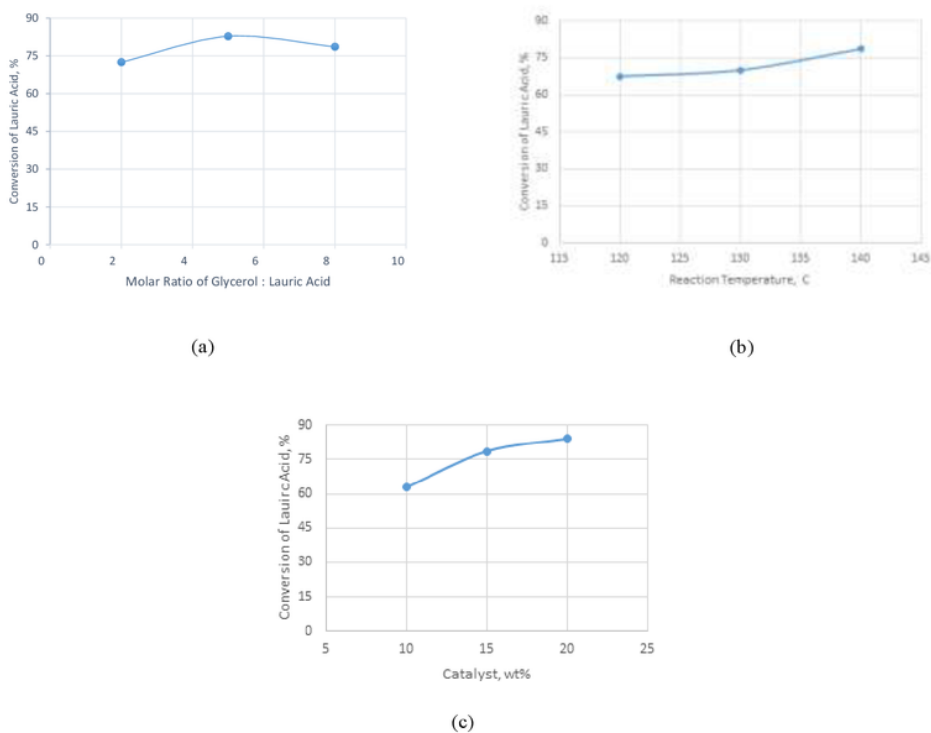
Figure 1. The effect of reaction conditions on reaction conversion
