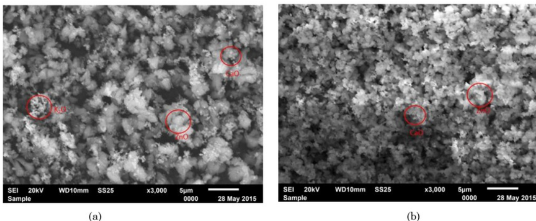
Figure 2. Scanning Electron Microscopy images of 2% \text{K}_2\text{O}/\text{CaO}-\text{ZnO} catalyst: (a) fresh catalyst; (b) after three cycles of used
