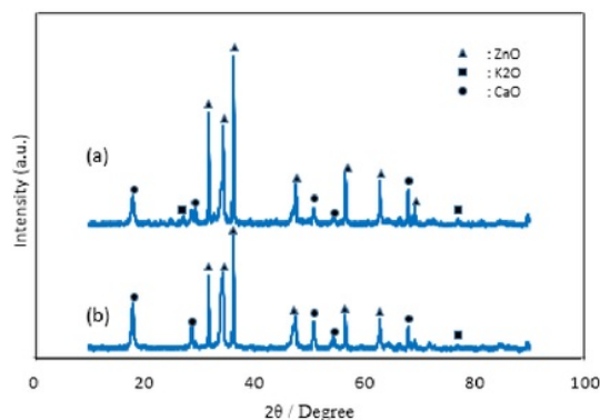
Figure 1. XRD pattern of catalysts: (a) Fresh catalyst of 2% K 2 O/CaO-ZnO, (b) Three cycles used catalyst of 2% K 2 O/CaO-ZnO
