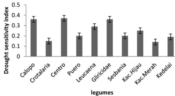
Figure 1 . Drought sensitivity index of ten legumes
