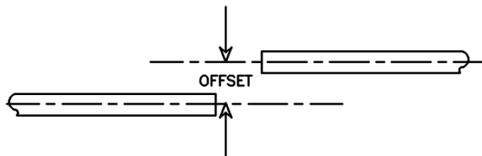
Gambar 2.12 Offset / Parallel Misalignment
