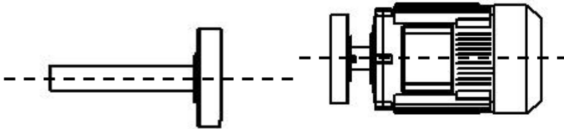
Gambar 2.15 Horizontal Misalignment
