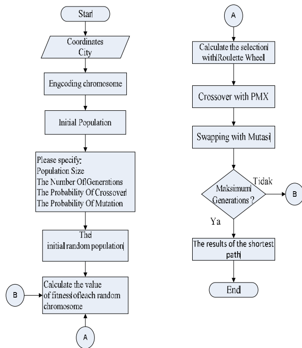
Figure 3.1 Genetic algorithm flowchart
