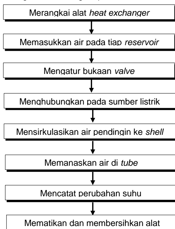
Gambar 2. Diagram Blok Prosedur Pengoperasian Alat Heat Exchanger
