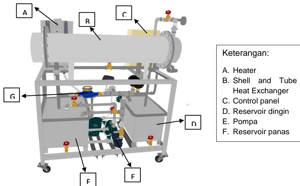
Gambar 1. Rangkaian alat shell and tube heat exchanger hasil perancangan
