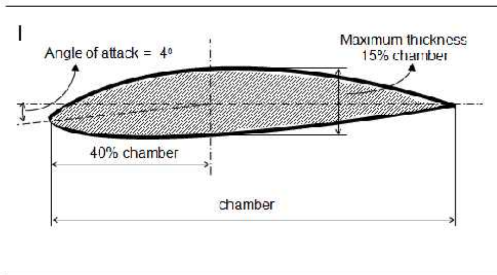
Gambar 2.3 Airfoil Naca 4415
