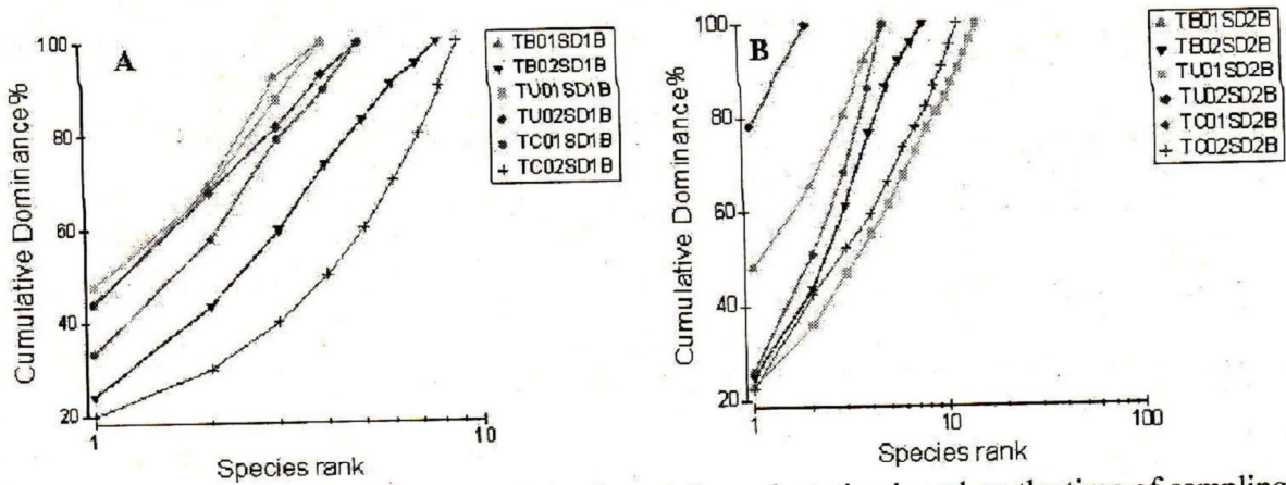
Figure 3. Cumulative k -dominance curves projected for each station based on the time of sampling: (A) Sampling I (July 2009), and (B) Sampling II (October 2009)
