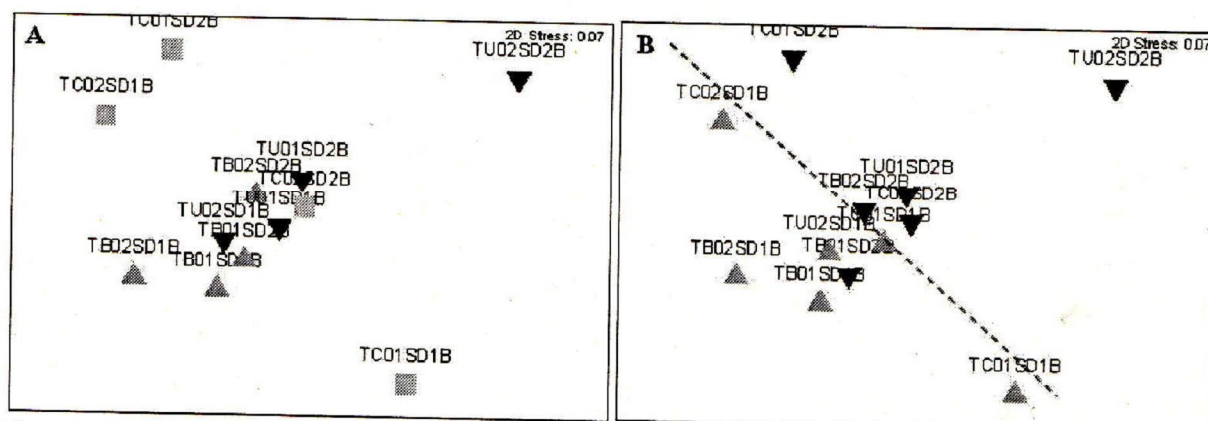
Figure 2. Ordination of Non-Metric Multidimensional Scaling (NMDS) projected based on Log (X+1) transformed data of categorised according to: (A) type of ponds: ▲ milkfish ponds; ▼ shrimp ponds, mixed ponds; ■ (B) sampling time: ▼ Sampling I, ■ Sampling II.
