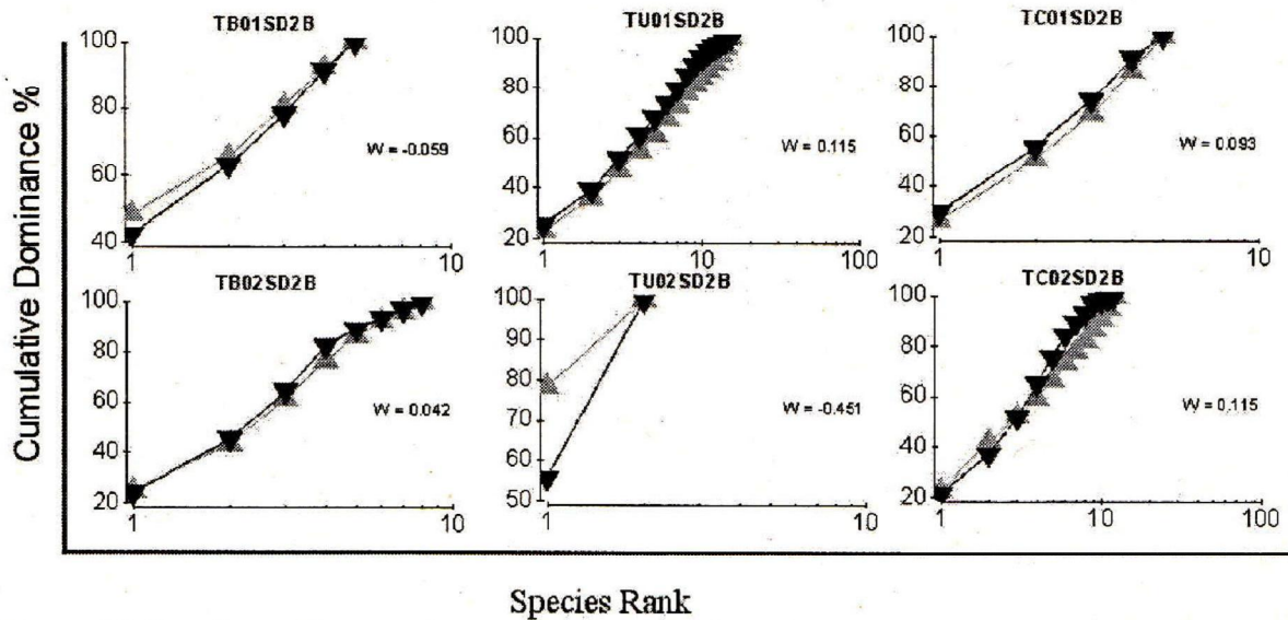
Figure 5. Abundance Biomass Curves Curve (ABC) is projected based on data transformation \log(X + 1) of abundance ( \blacktriangle ) and biomass ( \blacktriangledown ) macrobenthos in the second sampling time.
