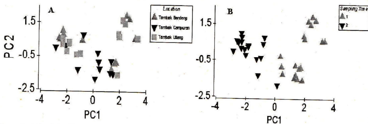
Figure 1. Principle Component Analysis (PCA) generated from the water parameter data, projected by: (A) Type of fishpond, (B) The time of sampling.
