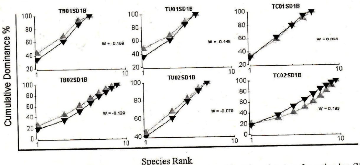
Figure 4. Abundance Biomass Curves Curve (ABC) is projected based on data transformation log (X +1) of abundance (▲) and biomass (▼) macrobenthos in the first sampling time.
