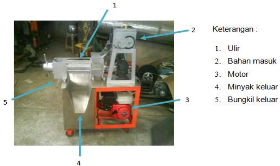
Gambar 6. Alat Screw Press
