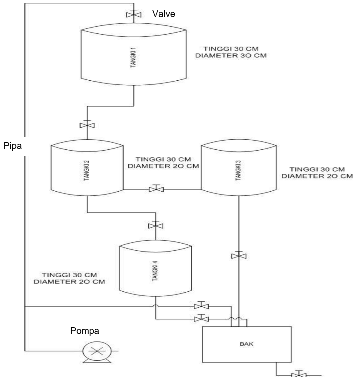
Gambar 4. Flow Chart Dinamika Proses (Anonim, 2015)
