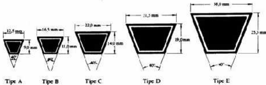
Gambar 2. 1 V-Belt Konvensional Tipe Standard
