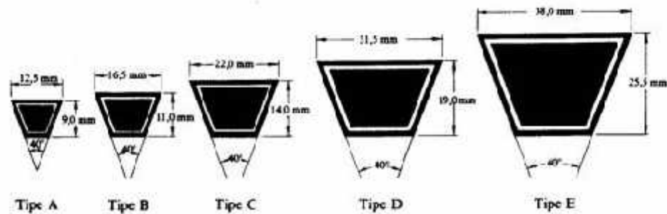
Gambar 2. 2 V-Belt Konvensional Tipe Standard
