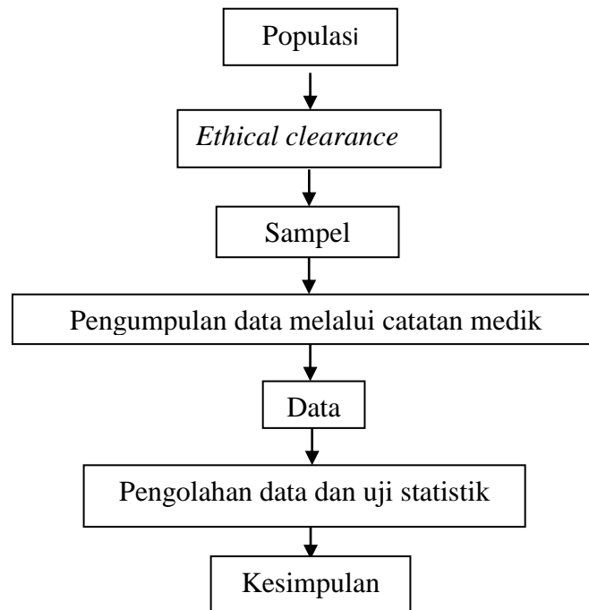
Gambar 3. Alur penelitian
