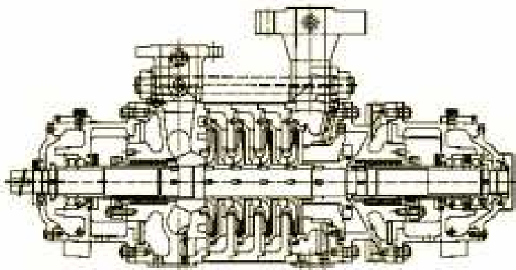
Gambar 2.9 Pompa Multistage
