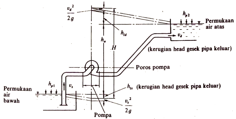
Gambar 2.11. Head Pompa
