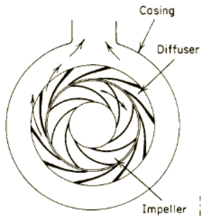
Gambar 2.8 Pompa diffuser
