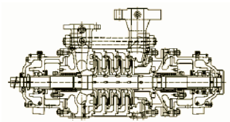
Gambar 2.9 Pompa Multistage
