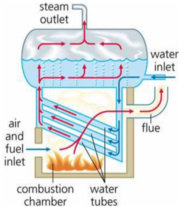
Gambar 2.2 Ketel Pipa Air (YourDitionary.com)
