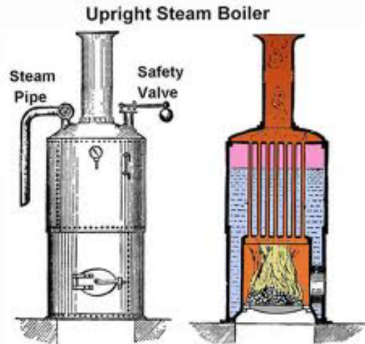
Gambar 2.3 Ketel Tegak (UNEP)
