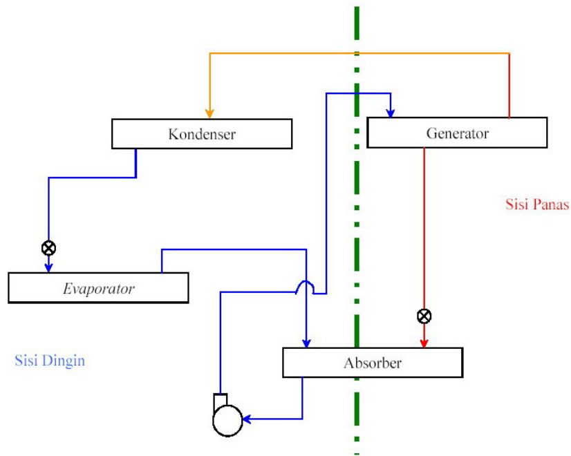
Gambar 2.7. Sistem refrigerasi absorbs (Sunyoto,2010)
