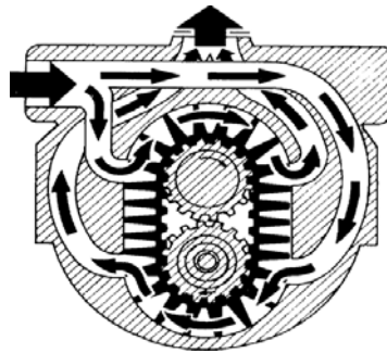
Gambar 2.4 Double Pump
