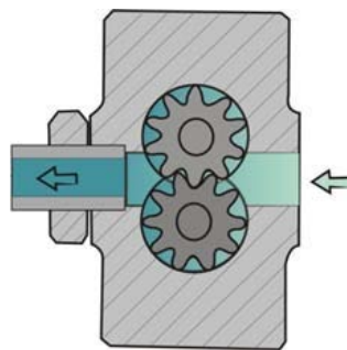
Gambar 2.5 Roda Gigi
