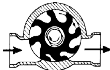
Gambar 2.3 Pompa Single-Stage Tekanan Rendah
