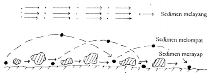
Gambar 2.5 Macam-Macam Pengangkutan Sedimen (Asdak 1995)
