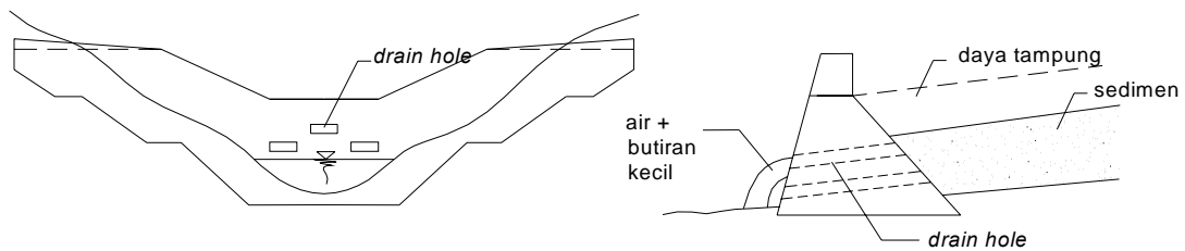
Gambar 2.24 Lubang Drainase/ Drain Hole
