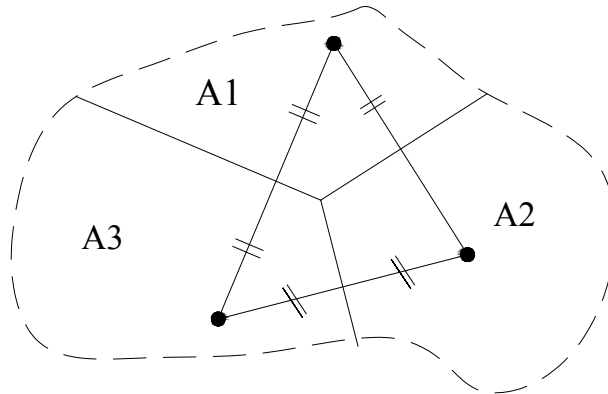
Gambar 2.7 Poligon Thiessen
