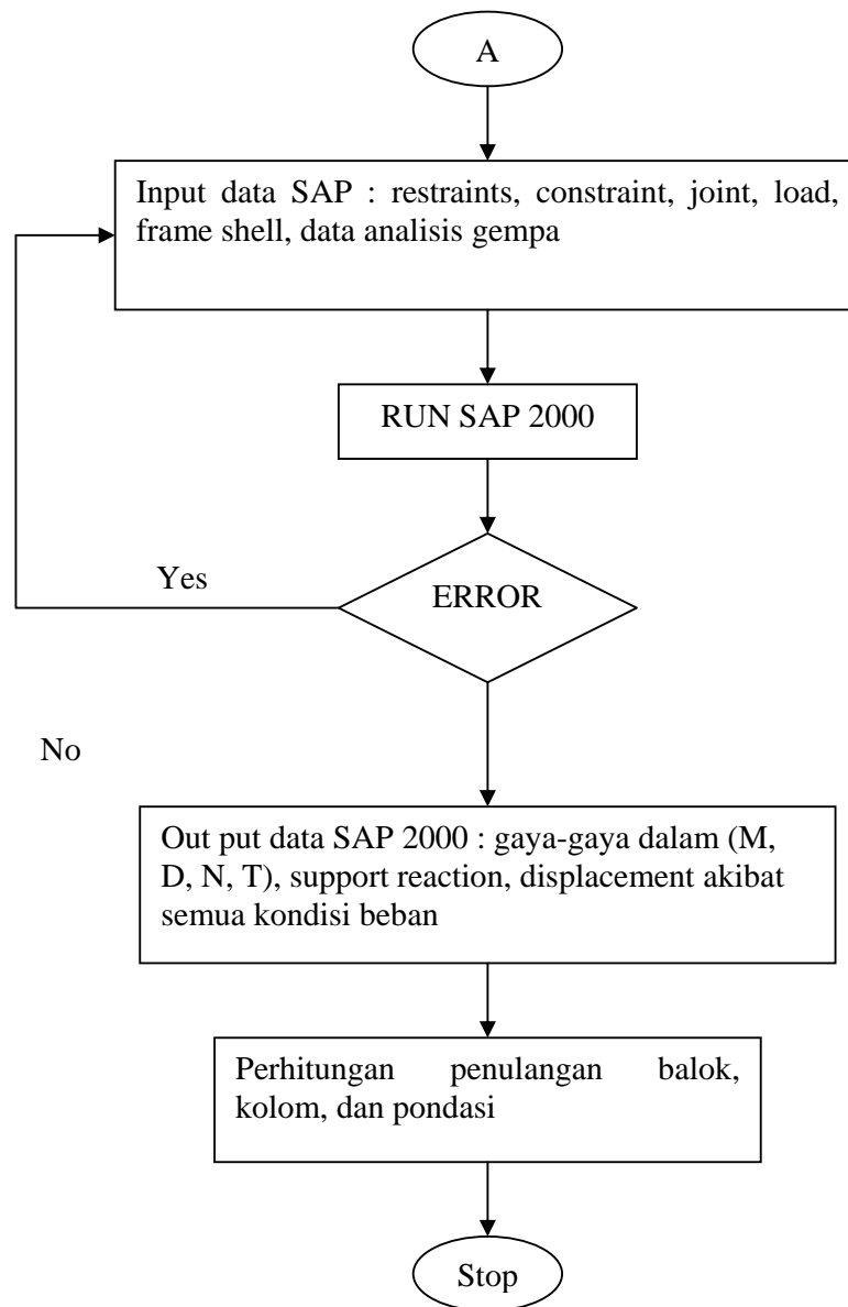
Gambar 3.2. Bagan Alir Perhitungan Mekanika Portal 3D
