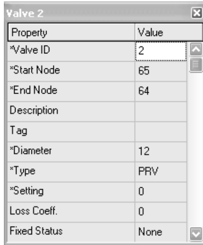
Gambar 2.14 Valve editor
