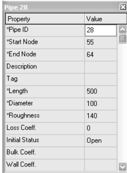
Gambar 2.12 Pipe editor
