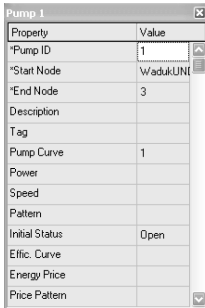
Gambar 2.13 Pump editor
