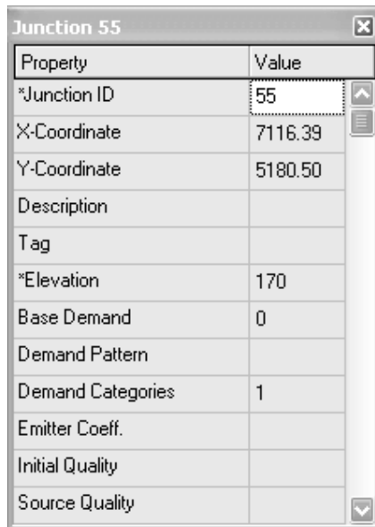
Gambar 2.9 junction editor
