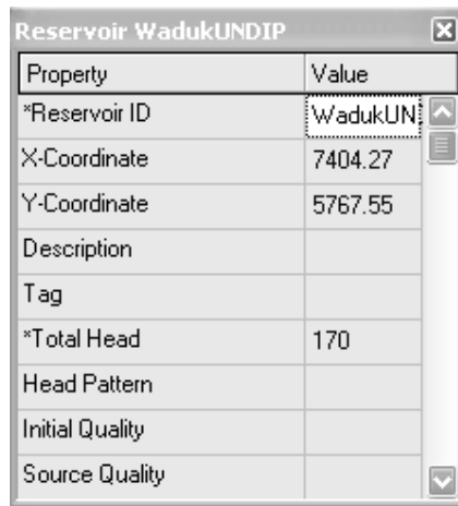
Gambar 2.10 resevoir editor
