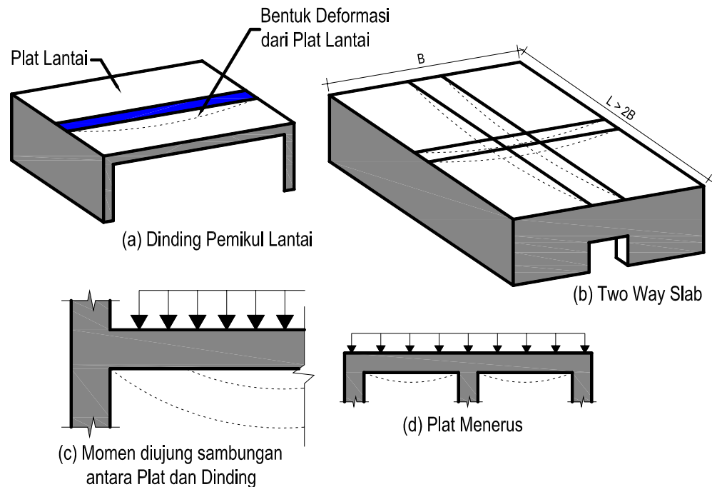
Gambar 2.1. Wall-supported slab systems.
