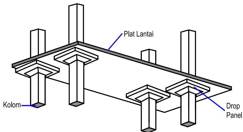
Gambar 2.5. Flat slab system
