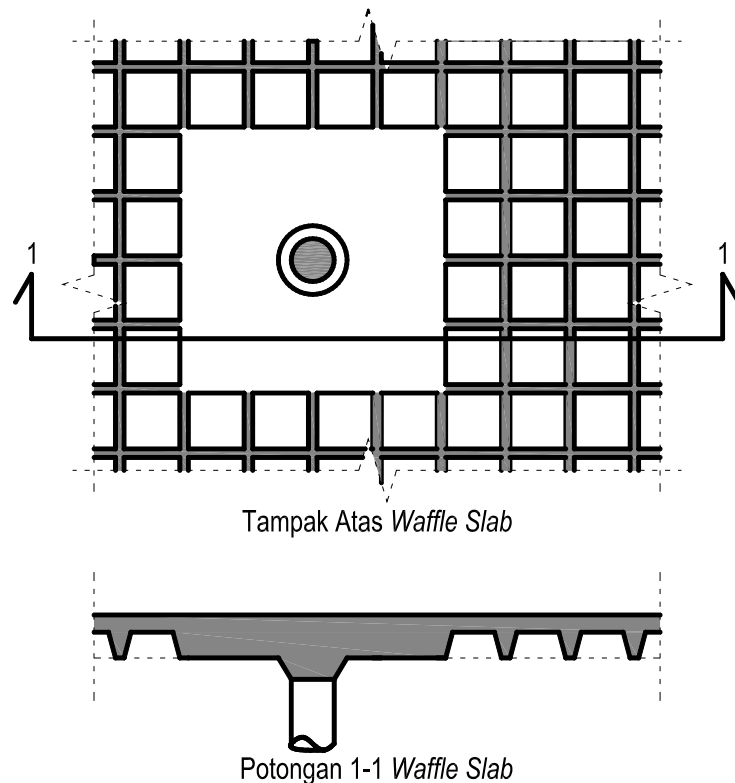
Gambar 2.3. Two-way ribbed slab system (Waffle Slab)
