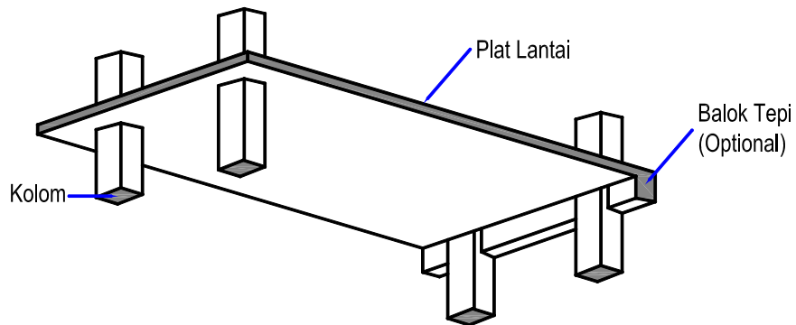
Gambar 2.4. Flat pelate system
