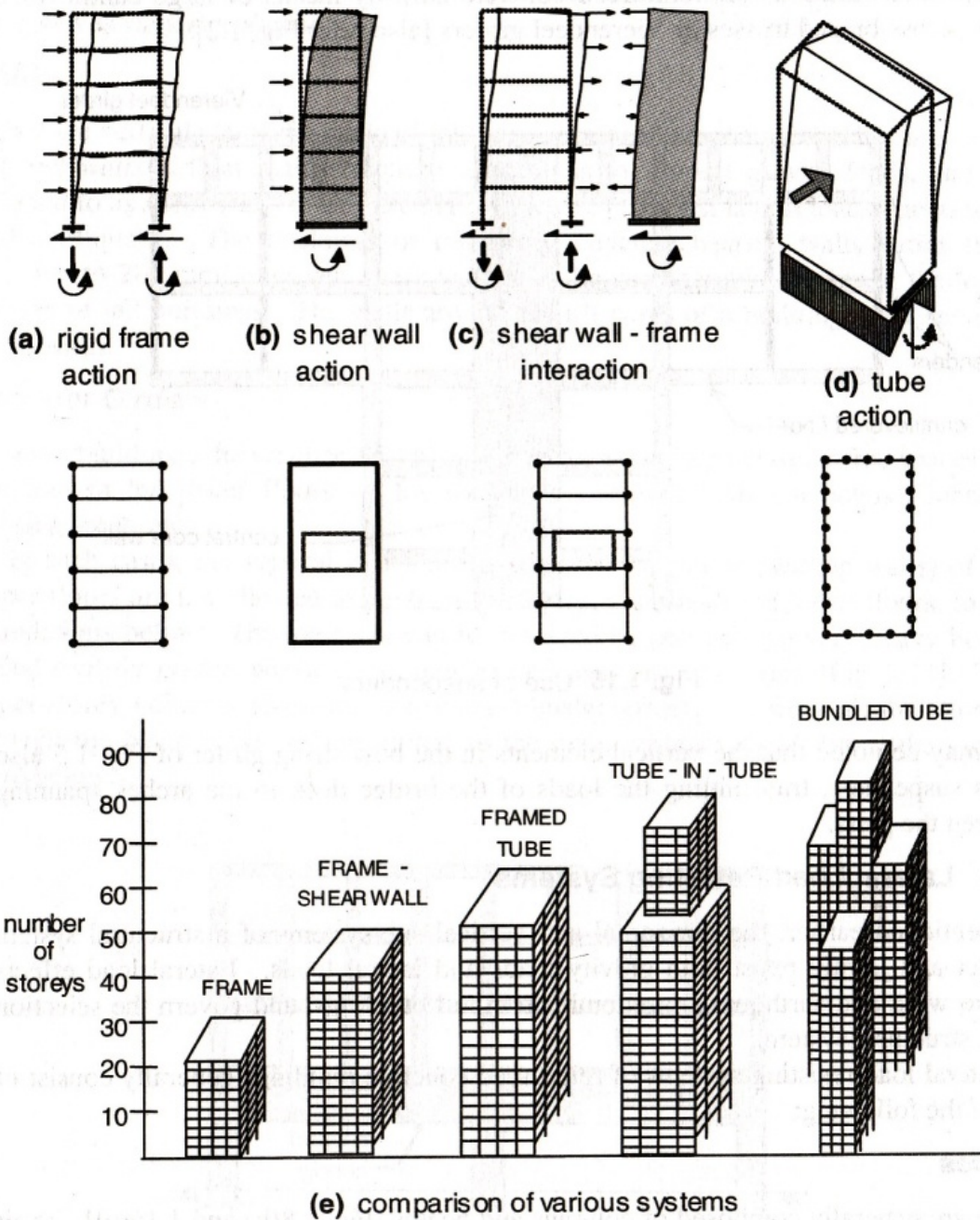
Gambar 2.8. Lateral Load Resisting System
