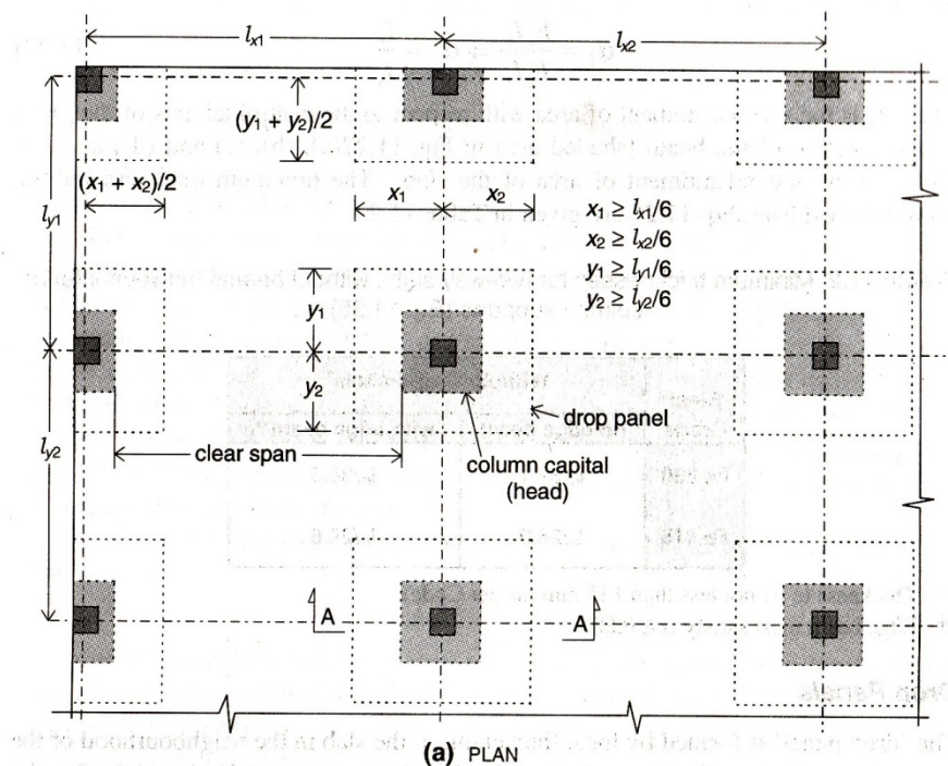
Gambar 2.27 Dimensi Drop Panel
