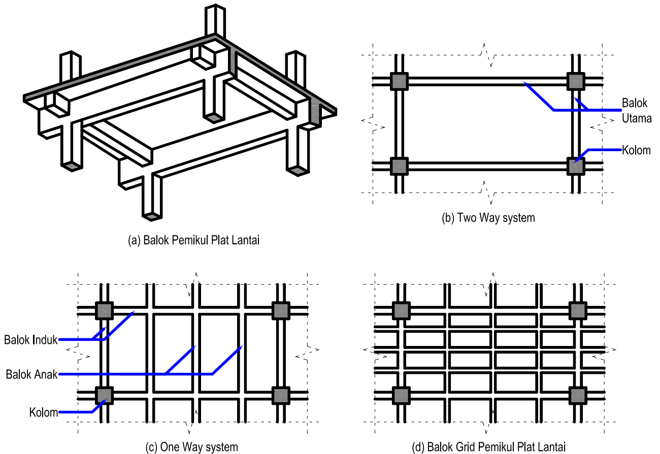
Gambar 2.2. Beam-supported slab system
