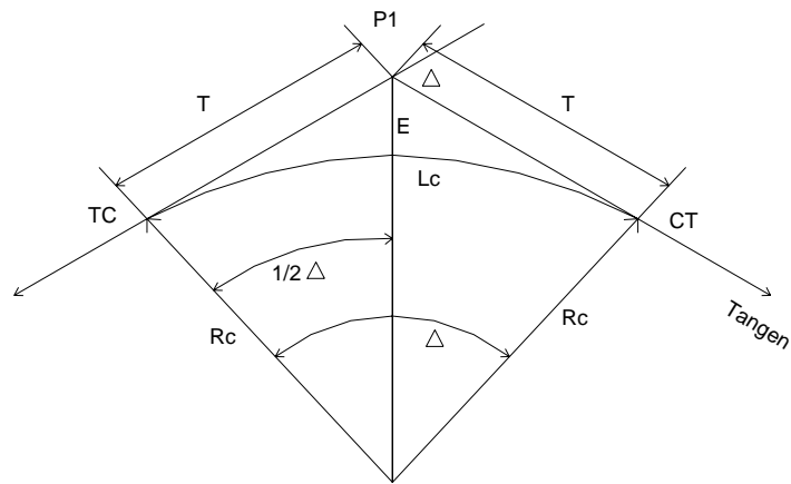
Gambar 2.1. Lengkung Full Circle
