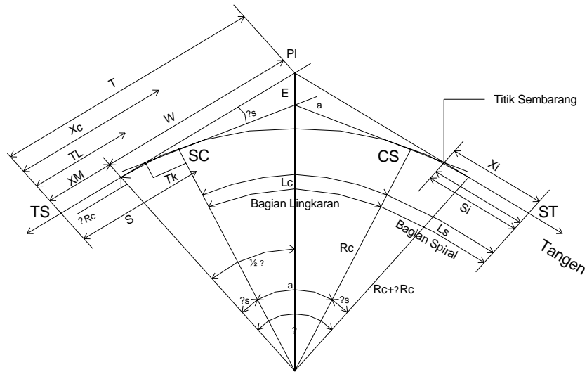
Gambar 2.2. Lengkung Spiral – Circle – Spiral
