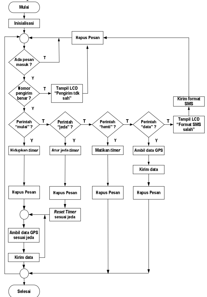
Gambar 3 Flowchart program utama.
