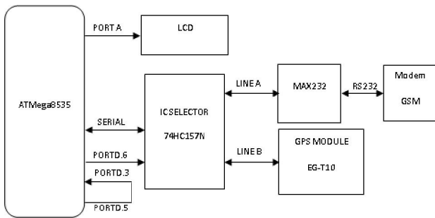
Gambar 2 Blok diagram hardware.
