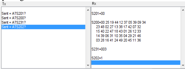
Gambar 6 Pengujian perintah AT Command 'ATSn?'
