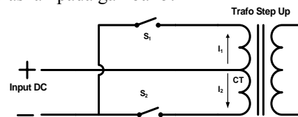
Gambar 5 Prinsip kerja inverter push pull
