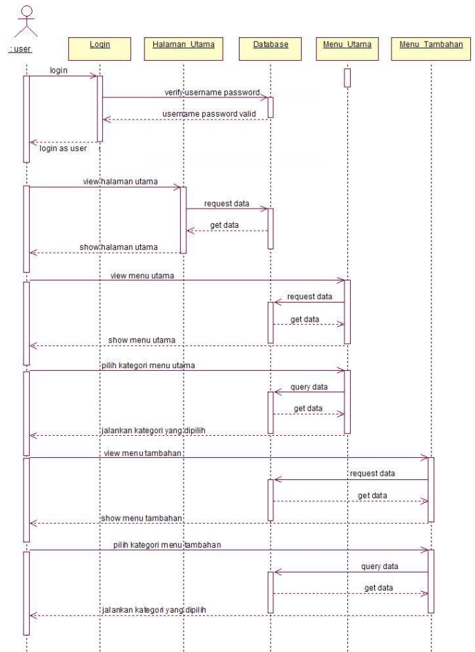
Gambar 7 Sequence diagram user terdaftar
