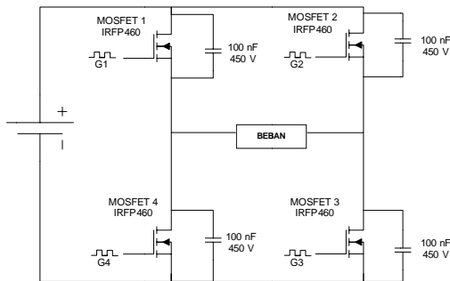
Gambar 15 Rangkaian inverter Full Bridge
