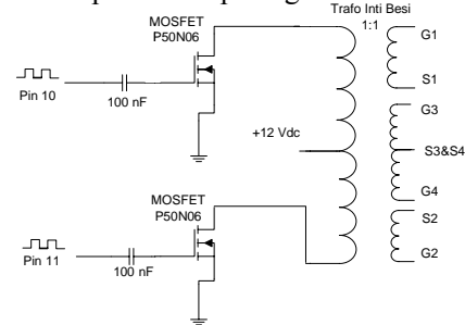
Gambar 17 Rangkaian driver dan trafo pulsa inti besi
