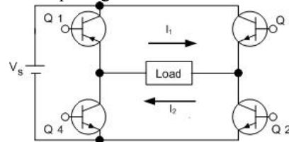
Gambar 6 Prinsip kerja inverter full bridge
