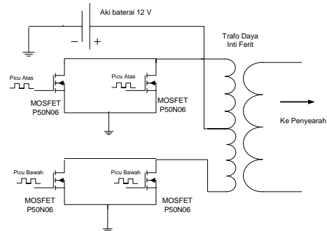
Gambar 10 Rangkaian inverter push pull
