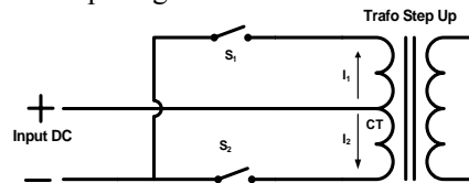
Gambar 5 Prinsip kerja inverter push pull
