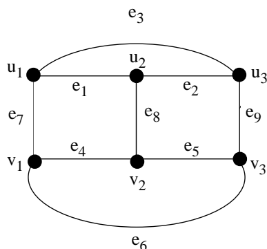
Gambar 2. Graph tangga L_3 .
