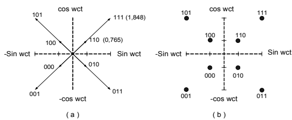
Gambar 2.1 Modulator 8-QAM : ( a ) diagram fasor, ( b ) diagram konstelasi.
