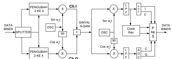
Gambar 3.1 Modulator dan demodulator 8-QAM.
