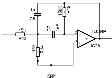
Gambar 3.11 Band pass filter 19 KHz.
