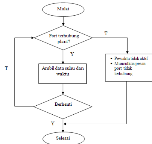
Gambar 3.3 Diagram alir prosedur simpan.
