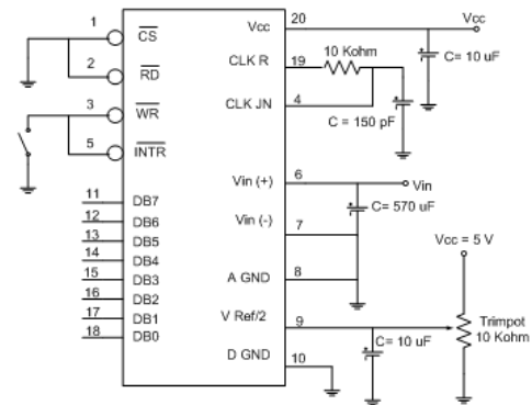
Gambar 2.2 Rangkaian free running ADC. [10]
