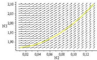
Figure 9. Trajectories for a system in N_2 - N_3 plane.
