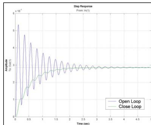
Gambar 4.6 Grafik Step Response
