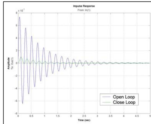
Gambar 4.5 Grafik Impulse Response
