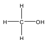
Gambar 6. Rumus kimia metanol ( \text{CH}_4\text{O} )
