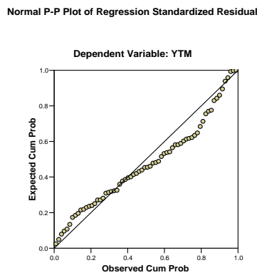
Gambar 4.3 Uji Normalitas ( normal probability plot )
