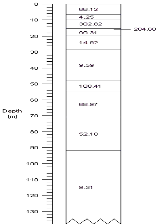
Gambar 9. Resistivity Log (Sunaryo, dkk, 2003).
