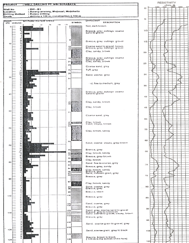
Gambar 10. Data Log/sonde (Sunaryo, dkk, 2003).
