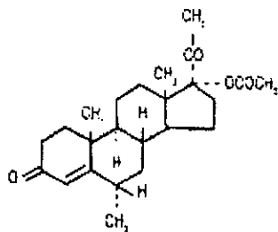
Medroxyprogesterone acetate
