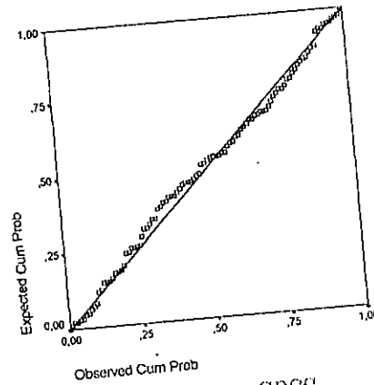
Gambar 4.2 HASIL UJI NORMALITAS NORMAL PROBABILITY PLOT
